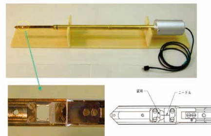
Fig.1 Electron microscope holder for nano-mechanical analysis.
