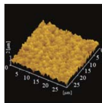
Figure 1: The surface of heat-resistant polymer (PEEK) exposed to space for 10 months. (Impingements of AO with a velocity of the International Space Station: 8km/s caused a severe damage to the surface.)
