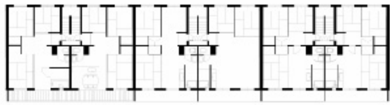
1F PLAN
