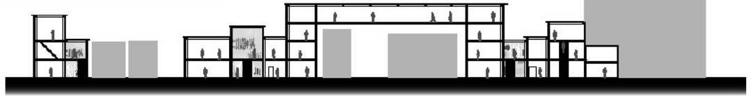
D-D' section
